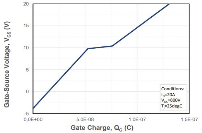
Figure 16. Gate Charge Characteristics
