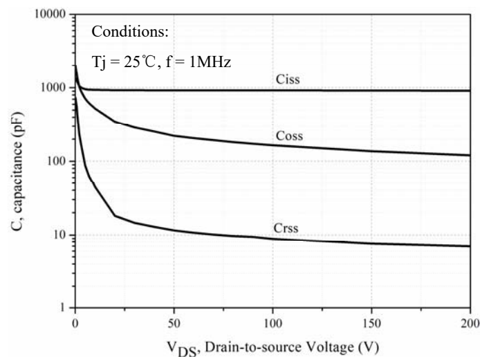
Figure 14. Capacitance vs. drain source voltage (0-200V)
