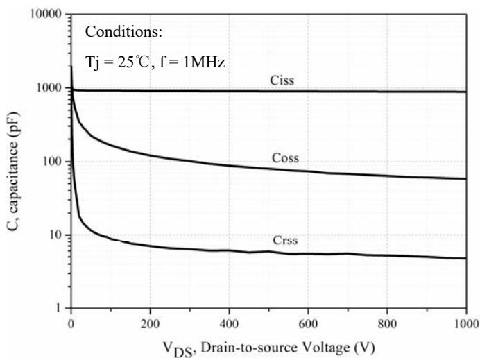
Figure 13. Capacitance vs. drain source voltage (0-1000V)
