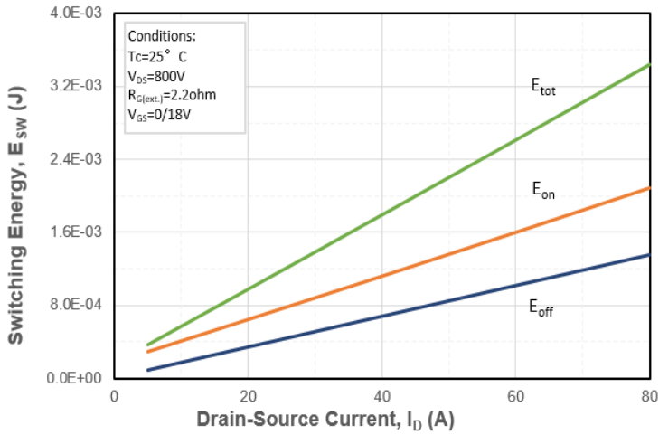
Figure 17. Clamped Inductive Switching Energy vs. Drain Current
