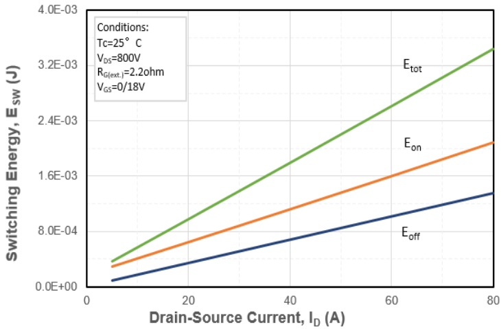
Figure 17. Clamped Inductive Switching Energy vs. Drain Current
