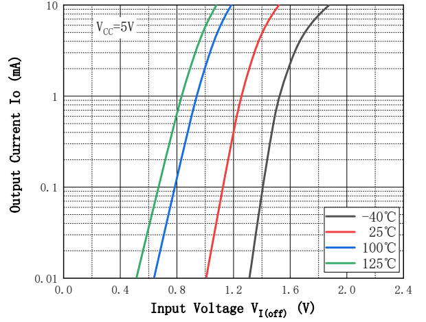
Fig.2 - OFF Characteristics
