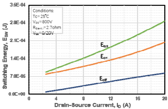
Figure 17. Clamped Inductive Switching Energy vs. Drain Current
