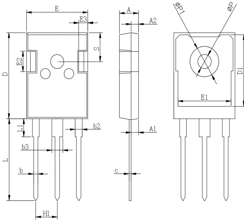
TO-247AB
