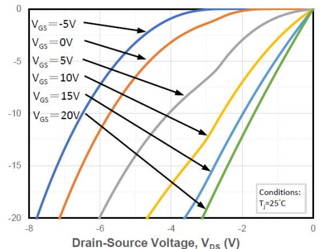
Figure 8. Reverse Output Characteristics at Tj = 25°C
